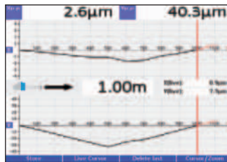
Straightness Measurement
