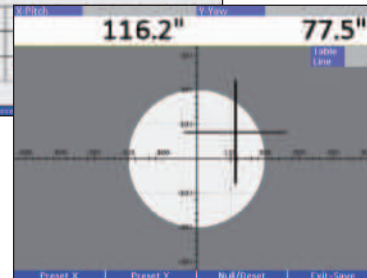
Input of tolerance limits and display of a circular tolerance field
