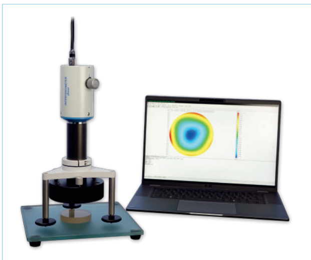
Fizeau Interferometer
